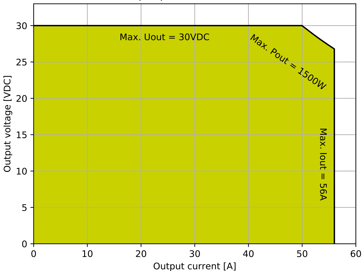
Output power characteristic
