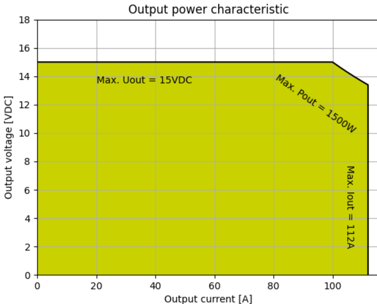
Figure 9.2: Output power DVCH1503-700-12
