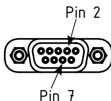
Abbildung 7.2: Pin assignment signal (CAN)
